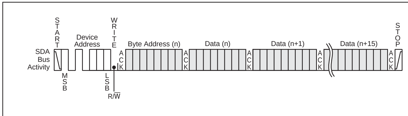
FIGURE 7. PAGE WRITE
