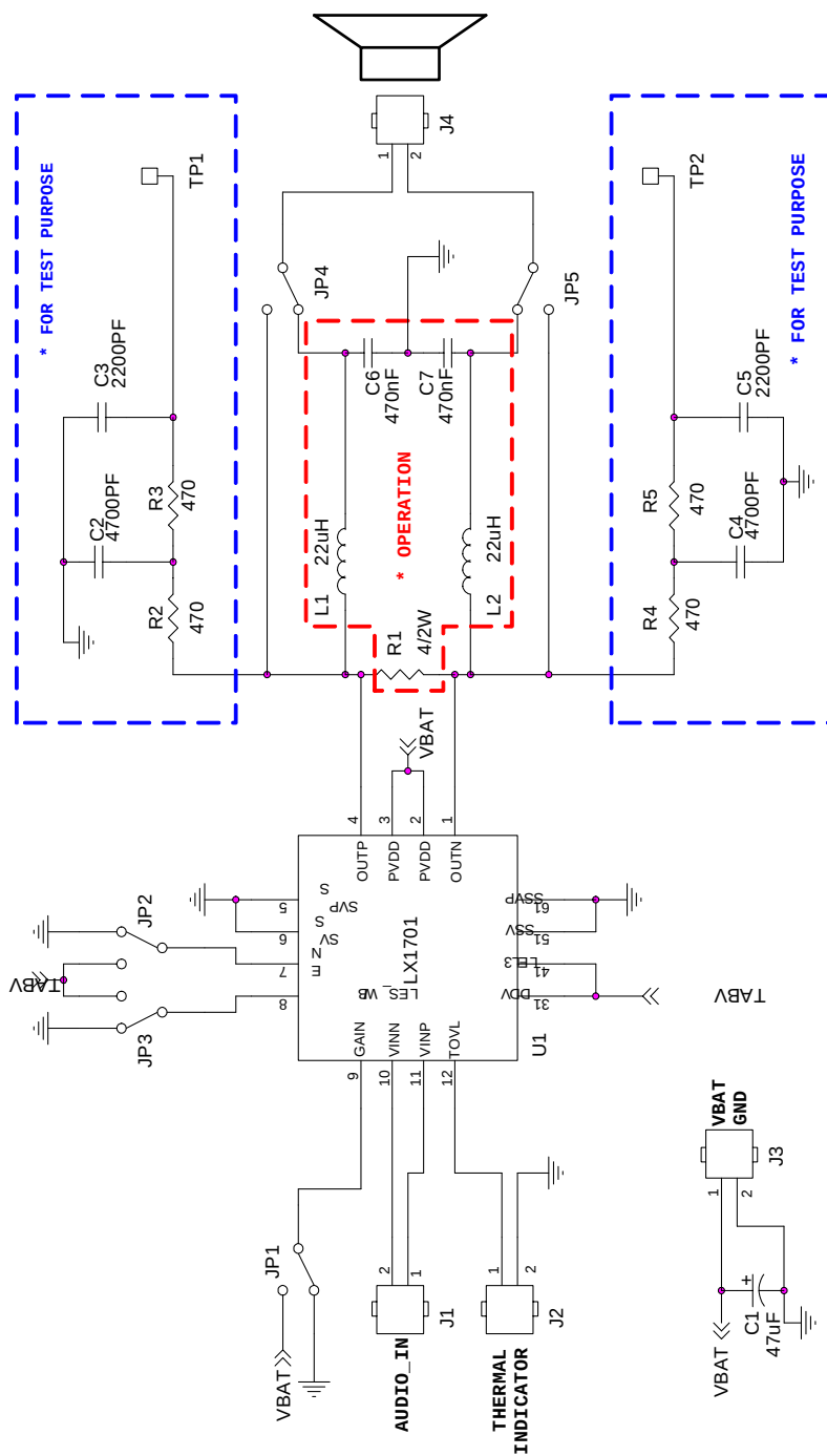
FIGURE 1 - LX1701 SCHEMATIC
