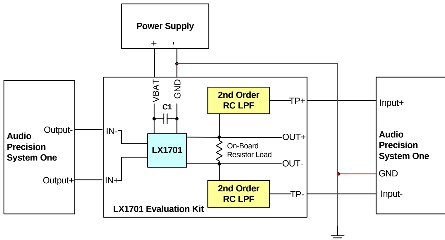
FIGURE 3 - LX1701 TEST SYSTEM SETUP
