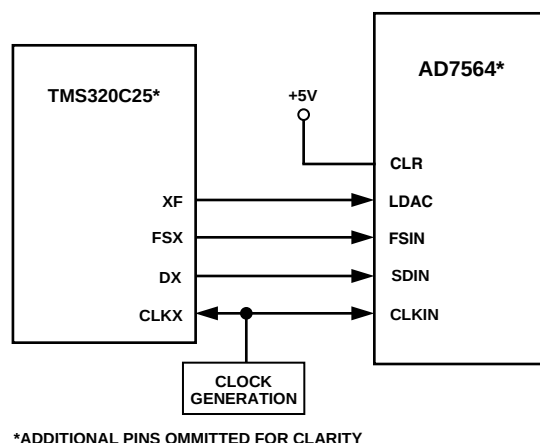
Figure 24. AD7564 to TMS320C25 Interface
