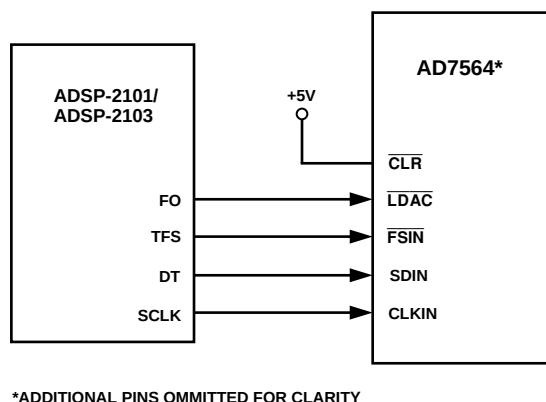
Figure 23. AD7564 to ADSP-2101/ADSP-2103 Interface
