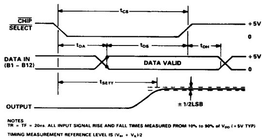
Figure 1. Timing Diagram
