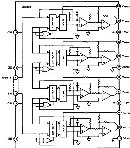
AD394 Functional Block Diagram
