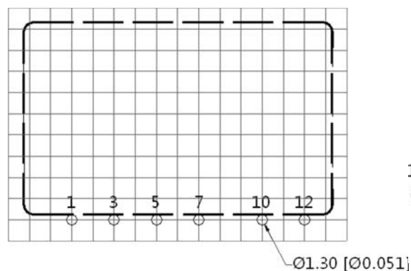
Top View PCB Layout
