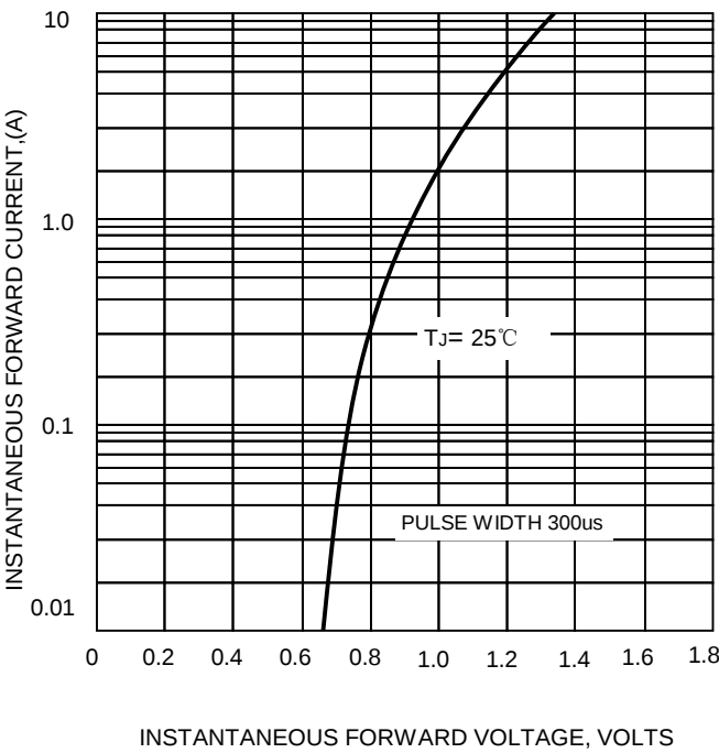
FIG.4-TYPICAL FORWARD CHARACTERISTICS
