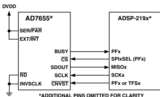
Figure 20. Interfacing the AD7655 to SPI Interface
