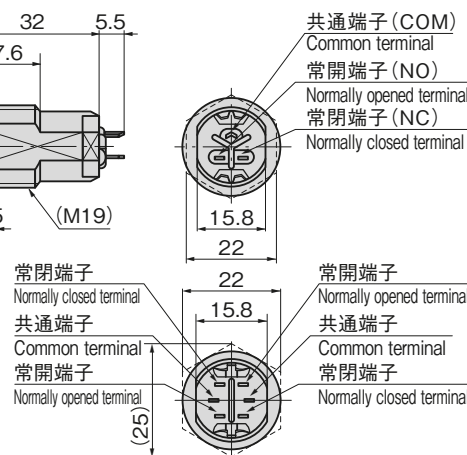
(2回路2接点型の裏面) (Back of two-circuit-two-contact type)
