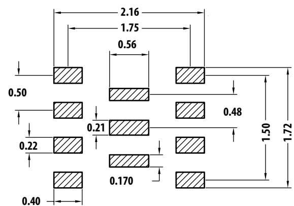
Stencil Opening
