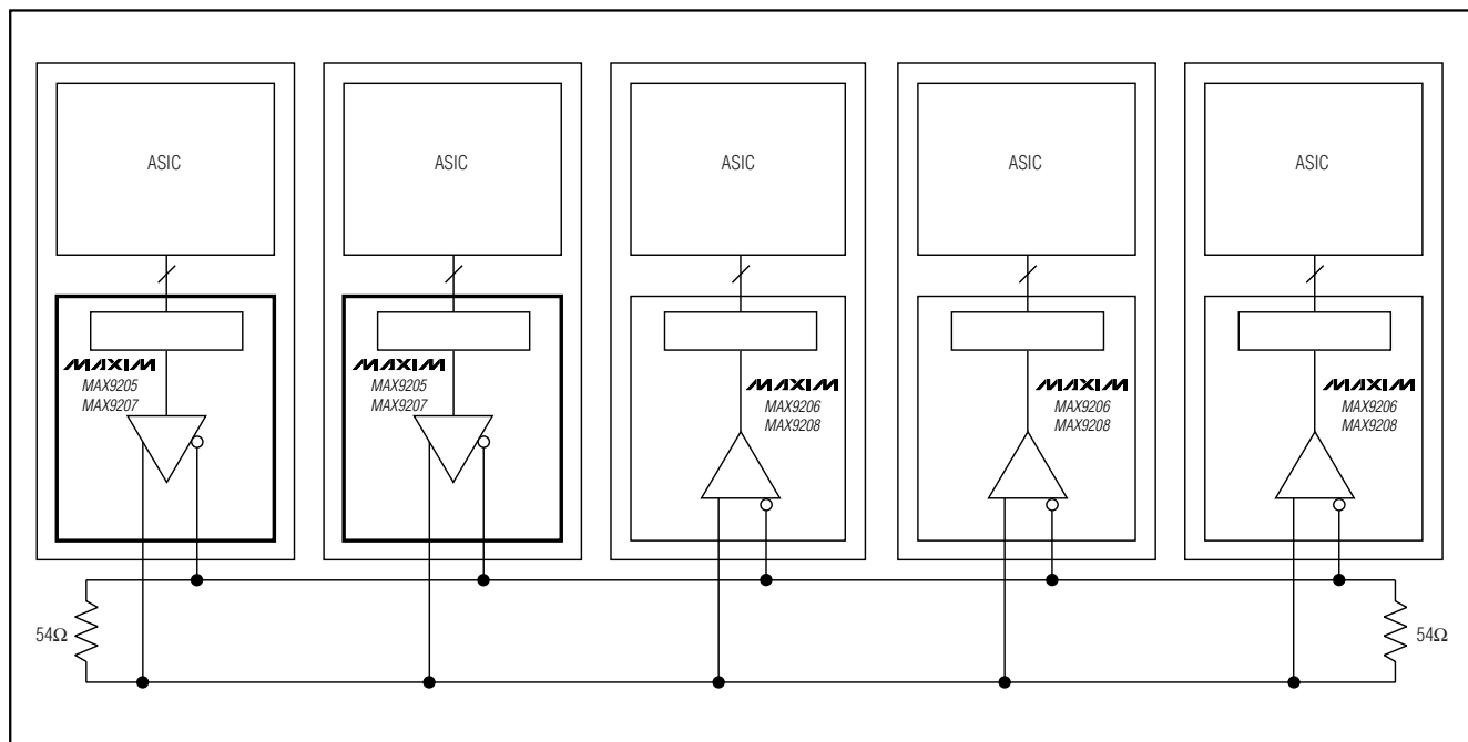
Figure 14. Multipoint
