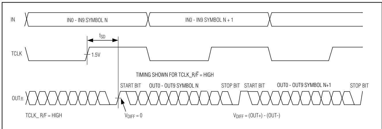
Figure 8. Serializer Delay
