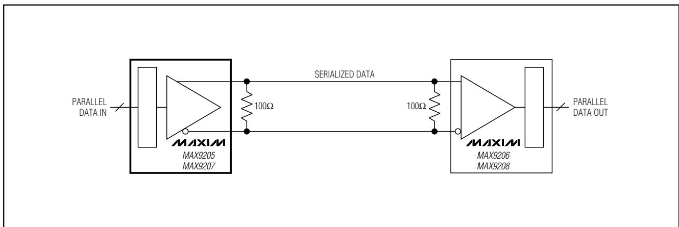
Figure 11. Double-Terminated Point-to-Point
