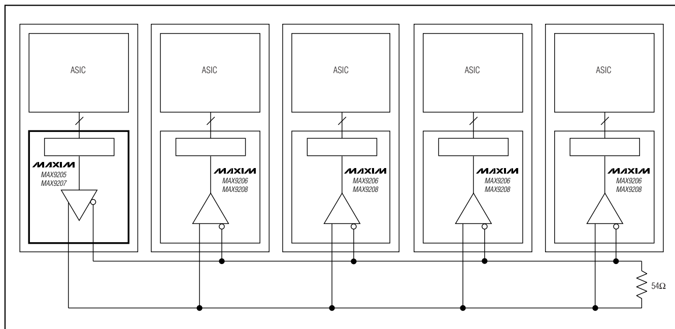
Figure 12. Multidrop
