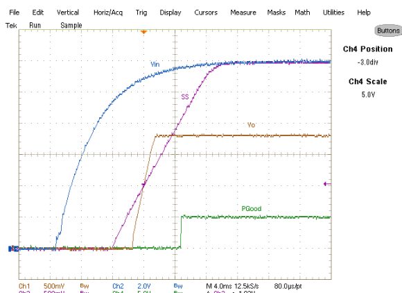
Fig. 8: Start up at 12A Load, Ch 1 :V o , Ch 2 :V in , Ch 3 :V SS , Ch 4 :V PGGood
