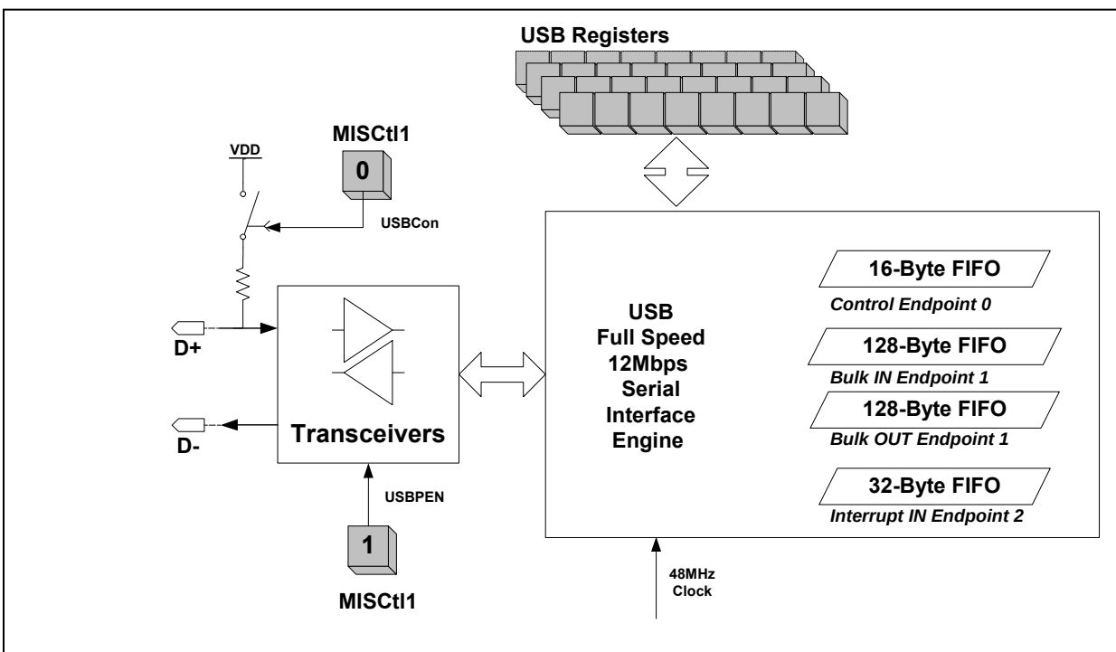
Figure 15: USB Block Diagram
