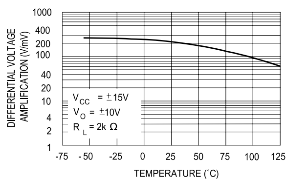
Figure 9: Large signal differential voltage amplification versus free air temperature
