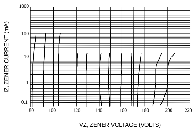
Fig. 9-ZENER VOLTAGE VERSUS ZENER CURRENT VZ = 82 THRU 200 VOLTS
