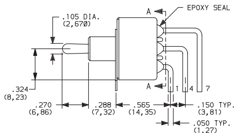
Actuator Shown In Pos. 1 .125 TYP. (3,18) Terminals & Support
