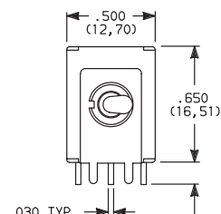
Actuator Shown In Pos. 1 .125 TYP. (3,18) Terminals & Support
