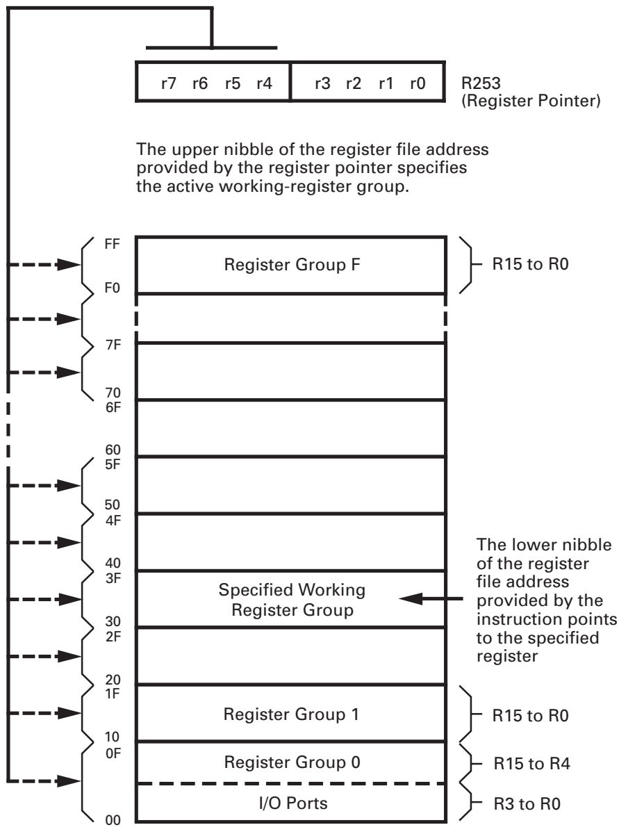
Figure 21. Register Pointer—Detail
