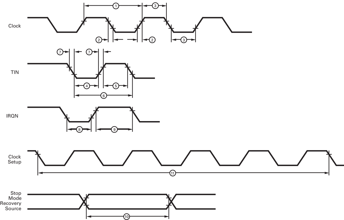
Figure 9. Additional Timing
