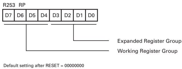
Figure 20. Register Pointer
