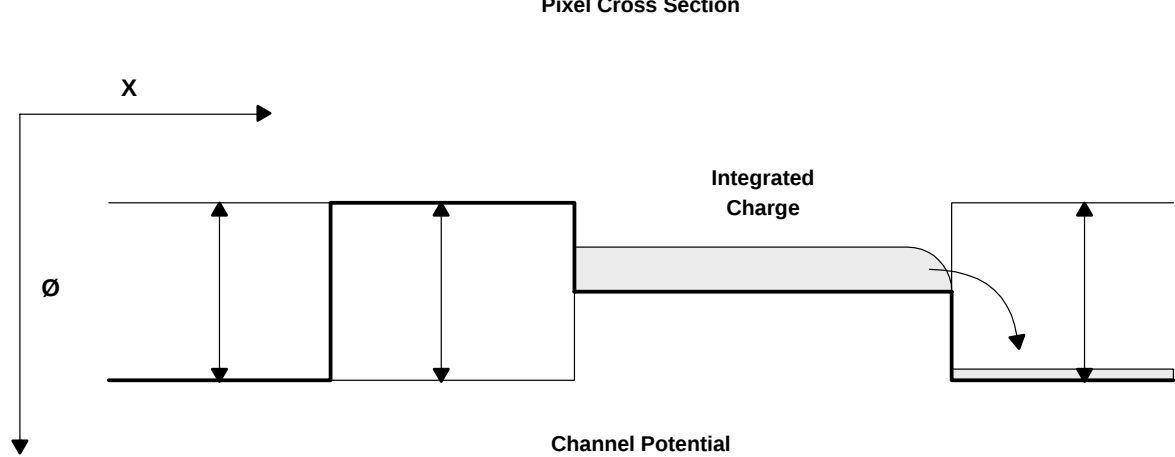
Figure 1. Image Area and Storage Area Pixel Cross Section with Channel Potential
