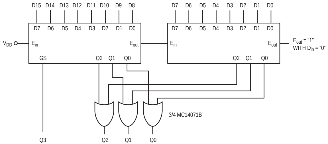
Figure 4. Two MC14532B's Cascaded for 4-Bit Output
