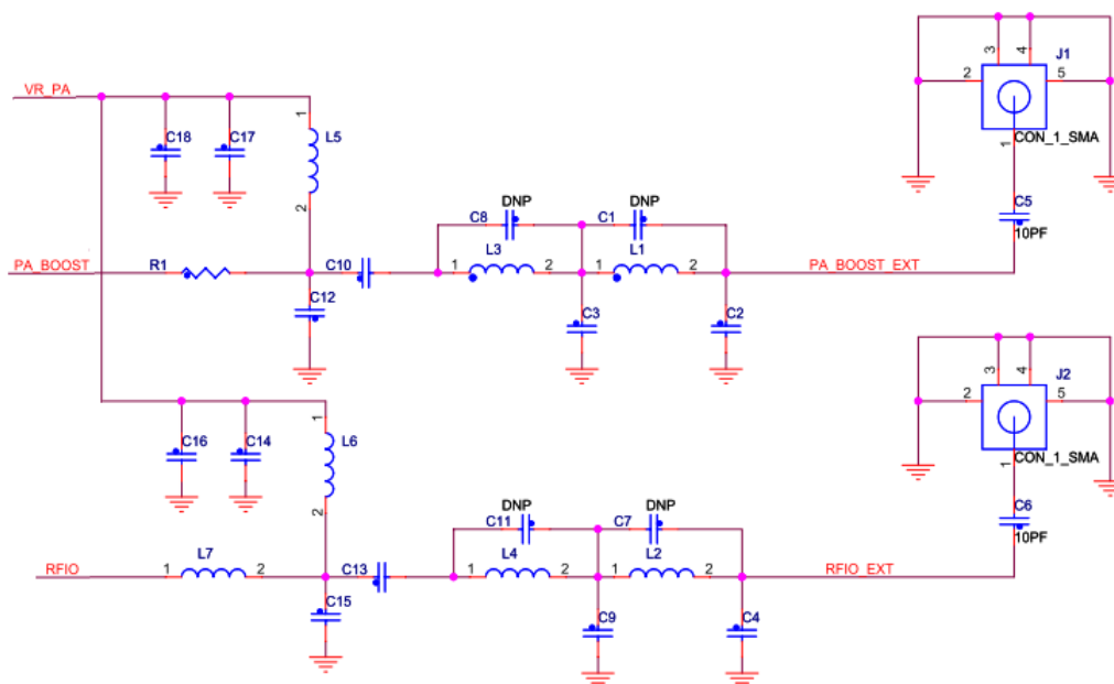
Figure 3-4. 12311-MRB RF Circuitry
