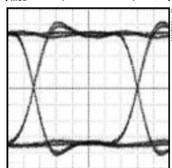
ELECTRICAL EYE DIAGRAM ( I_{MOD} = 25\text{mA} , 2^{13} - 1 + 80\text{ CID} , 32 QFN)
