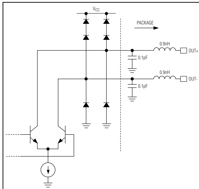
Figure 6. Simplified Output Circuit
