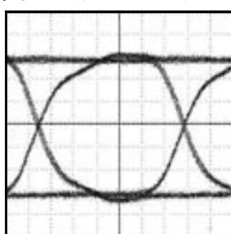
ELECTRICAL EYE DIAGRAM AC-COUPLED ( I_{MOD} = 80\text{mA} , 2^{13} - 1 + 80\text{ CID} , 32 QFN)
