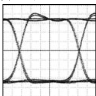
ELECTRICAL EYE DIAGRAM ( I_{MOD} = 60\text{mA} , 2^{13} - 1 + 80\text{ CID} , 32 QFN)
