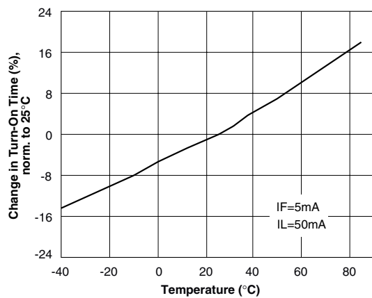
Figure 21. Turn-On Time vs. Temperature
