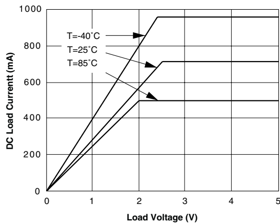
Figure 8. DC Current Limit vs. Temperature
