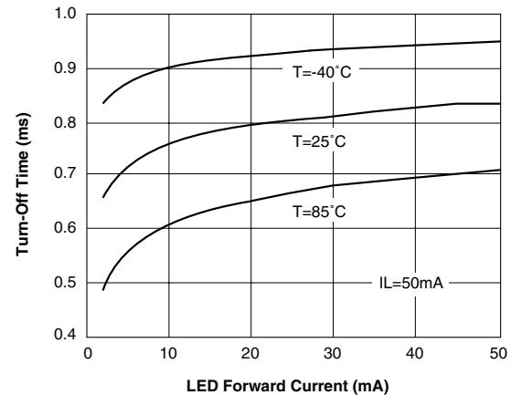
Figure 24. Turn-Off Time vs. LED Current
