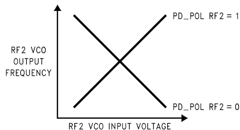
Figure 38. RF2 VCO Characteristics
