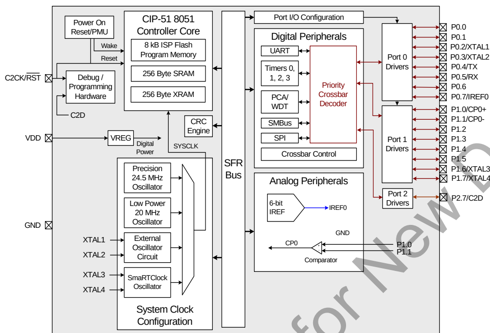
Figure 1.7. C8051F987 Block Diagram
