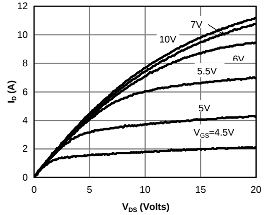
Figure 2: On-Region Characteristics@125°C
