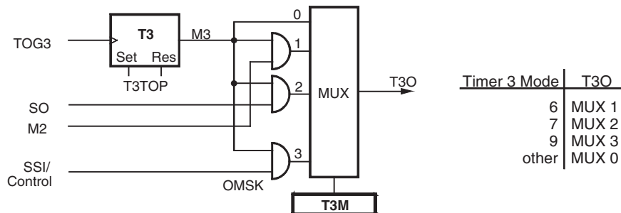
Figure 23-13. Modulator 3
