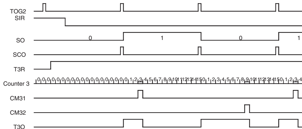
Figure 24-9. Pulse-width Modulation
