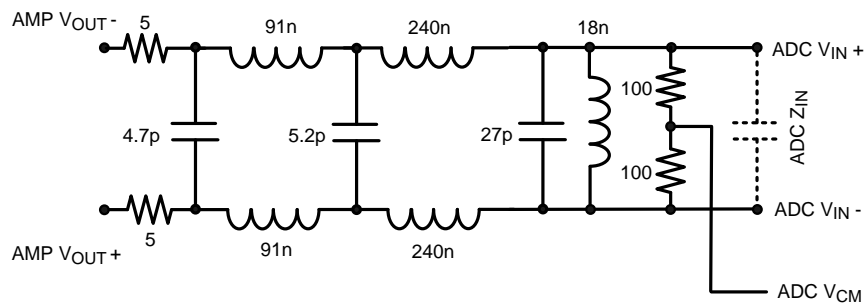
Figure 59. Impedance Transforming Filter 25 \Omega Input 210 \Omega Output, 210 MHz Center Frequency
