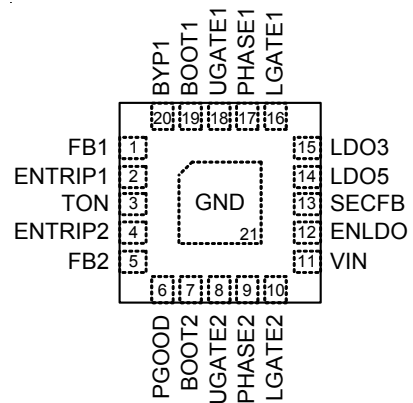
RT8239B/C
