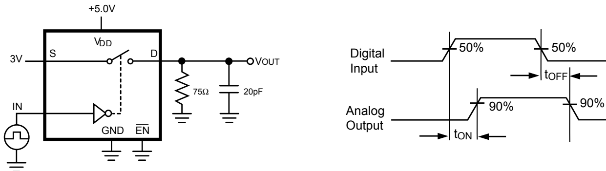
Figure 4. Switching Time
