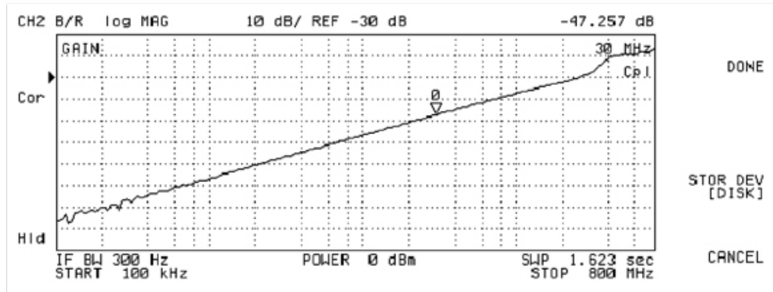
Figure 3. Crosstalk vs Frequency
