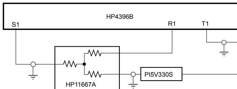
Figure 5. Gain/Phase, Crosstalk, Off-Isolation
