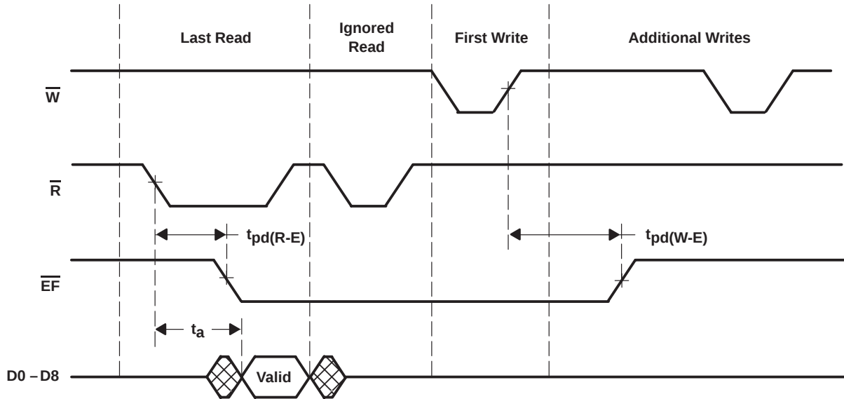
Figure 3. Empty-Flag Waveforms
