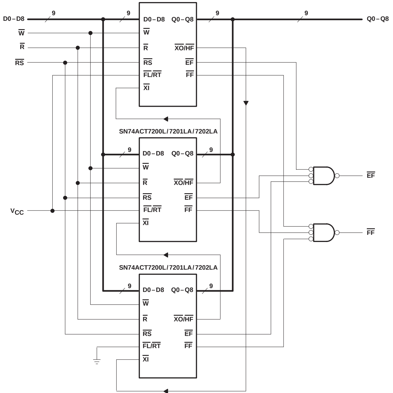
Figure 15. Word-Depth Expansion: 768/1536/3072 Words \times 9 Bits
