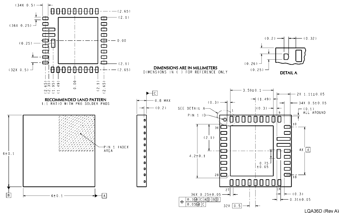
Leadless Leadframe Package (NS Package Number LQA036D), D Version (Bottom View) (LMX2531LQ1146E/1226E/1312E/1415E/1515E/2820E/3010E) Order Number LMX2531LQX for 2500 Unit Reel Order Number LMX2531LQ for 250 Unit Reel
