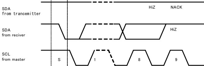
Figure 3 Start/End condition
