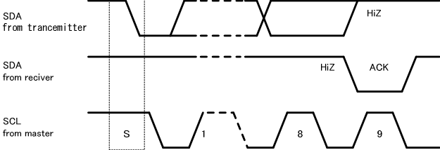
Figure 3 Start/End condition
