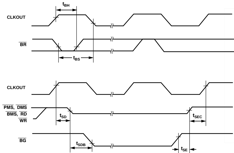
Figure 21. Bus Request/Grant
