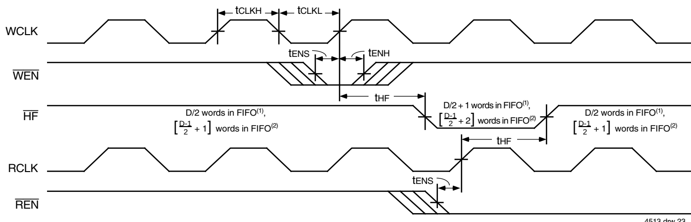
Figure 19. Programmable Almost-Empty Flag Timing (IDT Standard and FWFT Modes)
