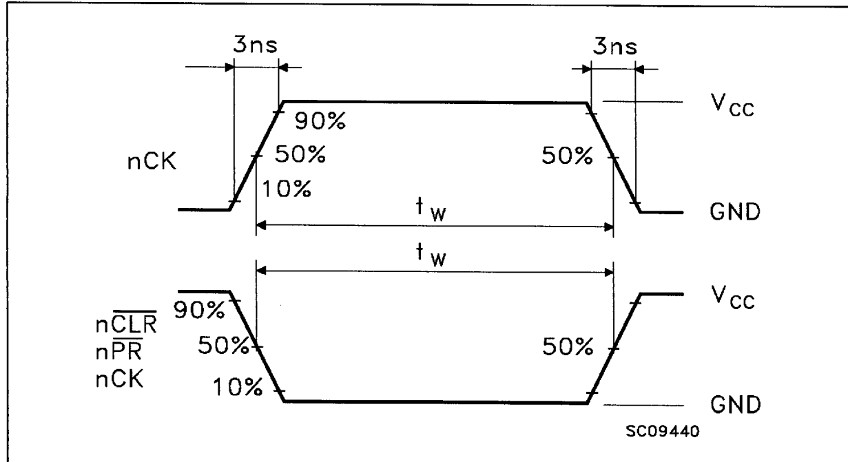
WAVEFORM 3: PULSE WIDTH
