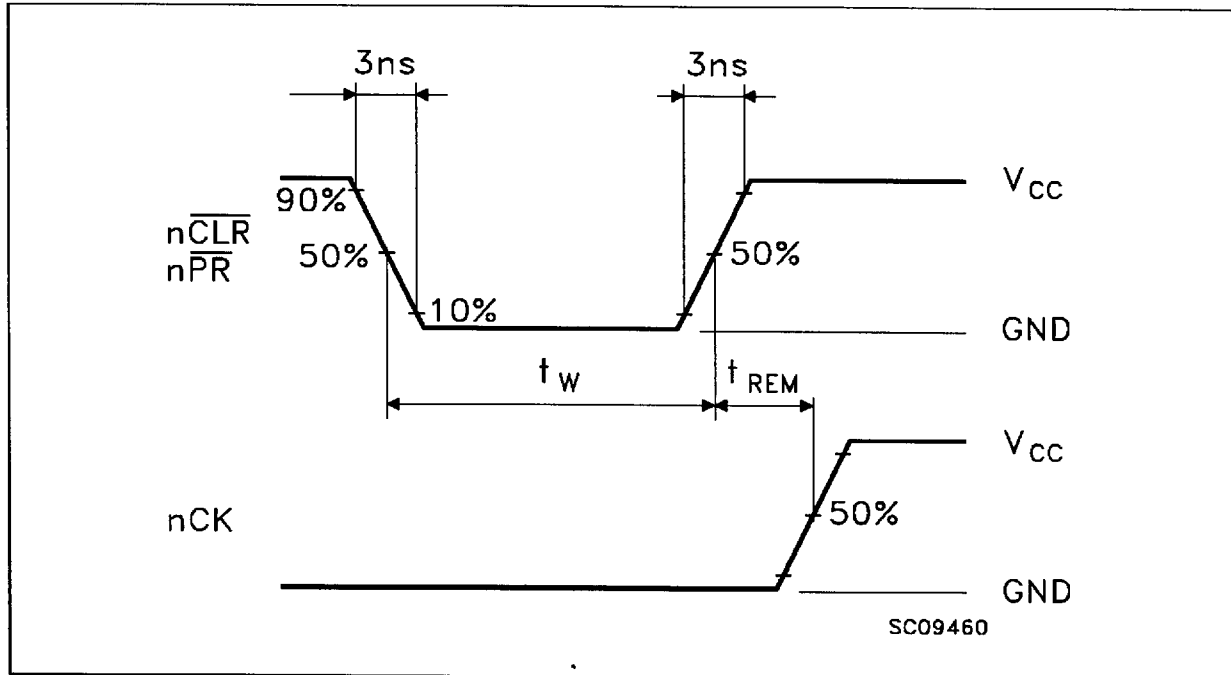
WAVEFORM 3: RECOVERY TIMES ( f=1\text{MHz} ; 50% duty cycle)
