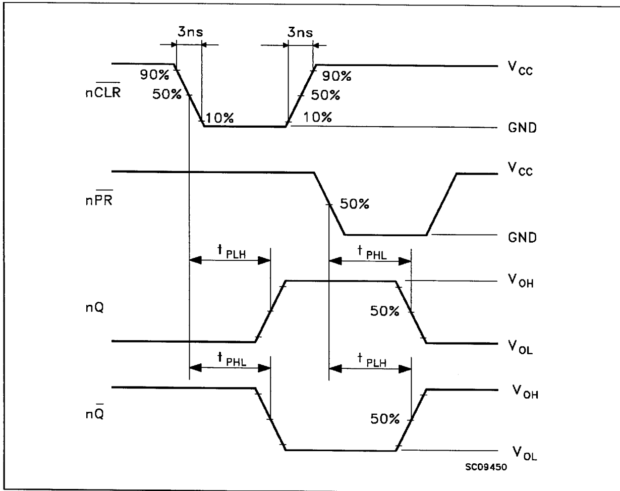
WAVEFORM 2: PROPAGATION DELAYS ( f=1\text{MHz} ; 50% duty cycle)
