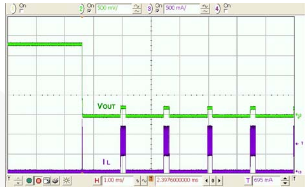
Figure 28. Over-Current, Load Increasing Past Current Limit, FAN53601 Figure 29. 250 mΩ Fault, Rapid Fault, Hiccup, FAN53601
