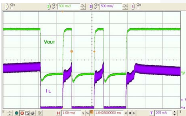
Figure 30. Over-Current, Load Increasing Past Current Limit, FAN53611 Figure 31. 250 mΩ Fault, Rapid Fault, Hiccup, FAN53611
