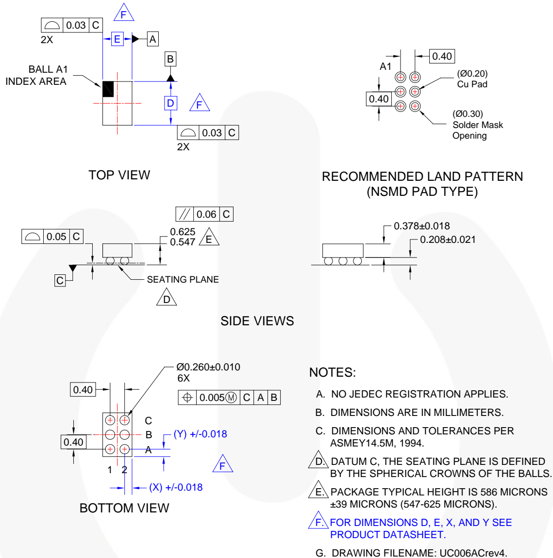
Figure 36. 6-Bump WLCSP, 0.4 mm Pitch
