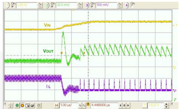
Figure 23. Combined Line / Load Transient, 3.3-3.9 V_{IN} , 10 \mu\text{s} Edge, 400-36 mA Load, 100 ns Edge 3.9-3.3 V_{IN} , 10 \mu\text{s} Edge
