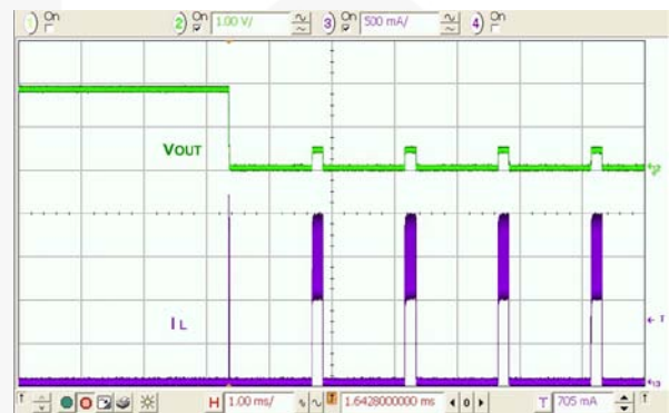
Figure 30. Over-Current, Load Increasing Past Current Limit, FAN53611 Figure 31. 250 mΩ Fault, Rapid Fault, Hiccup, FAN53611
