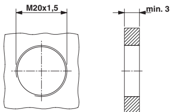
Dimensioned drawing
