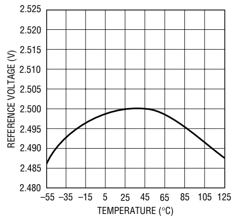
Temperature Drift
