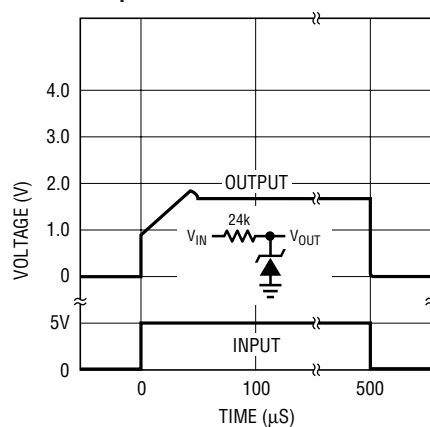
Response Time
