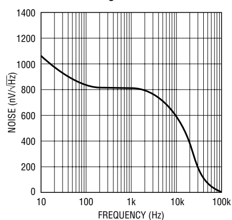
Noise Voltage
