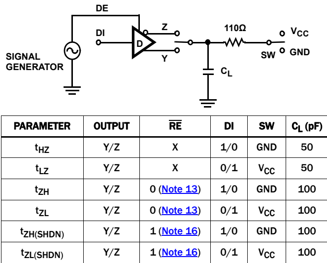
FIGURE 8A. TEST CIRCUIT
