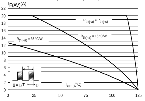
Figure 2: Average forward current versus ambient temperature ( \delta = 1 )
