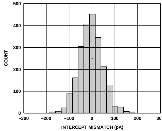
Figure 31. Distribution of Channel-to-Channel Intercept Mismatch ( I_{I1} - I_{I2} )
