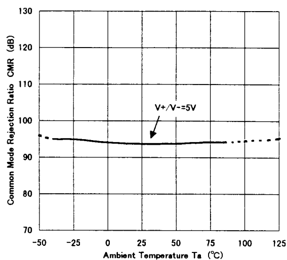
NJM14558 Common Mode Rejection Ratio vs. Temperature
