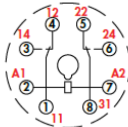
NEMA IEC Wiring Diagram Bottom View
