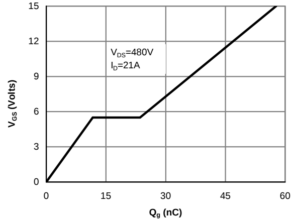
Figure 8: Gate-Charge Characteristics
