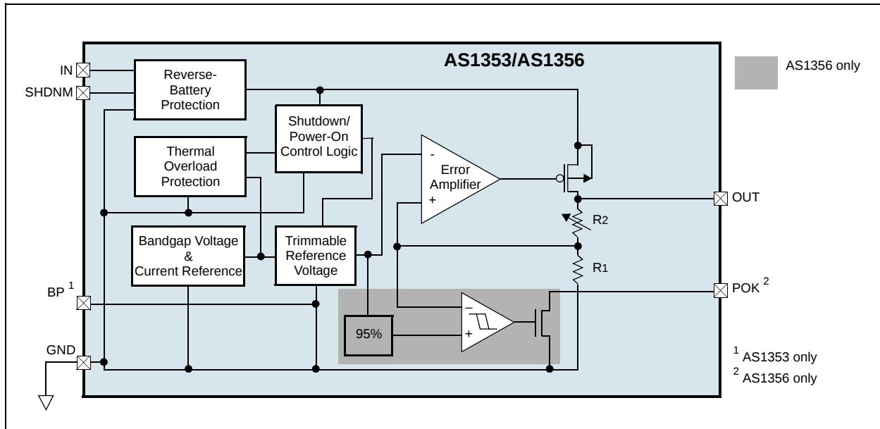
Figure 12. Block Diagram
