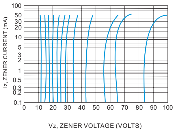
Fig.8 V_z = 12 thru 82 Volts
