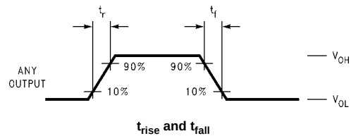
FIGURE 2. Waveforms (Input Pulse Characteristics; f=1\text{MHz} , t_r=t_f=3\text{ns} )
