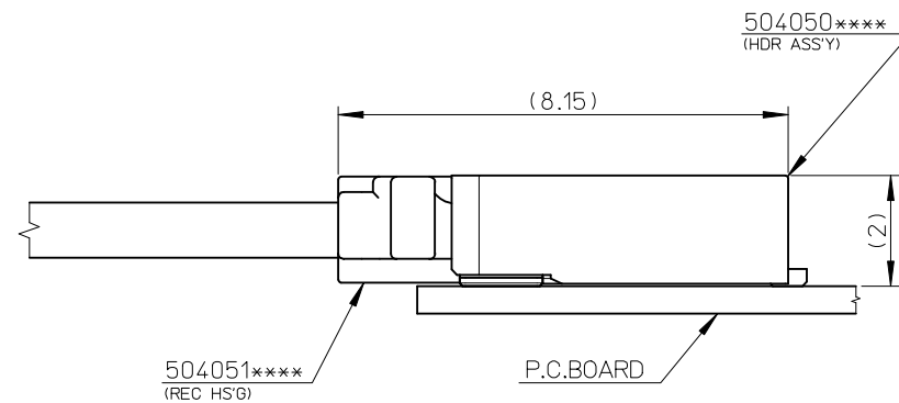
MATED CONNECTORS
