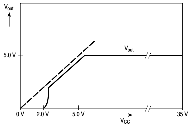
Figure 16. Output Voltage versus Supply Voltage
