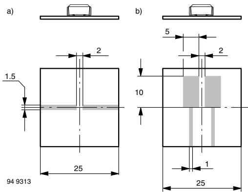
Figure 1. Boards for R_{thJA} Definition (Copper Overlay 35\text{ }\mu\text{m} )
