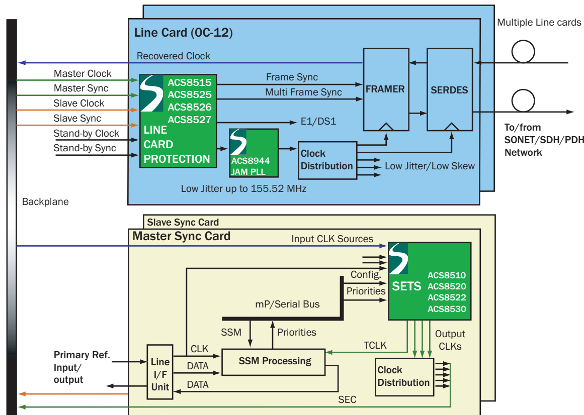
Figure 10 Typical Application
